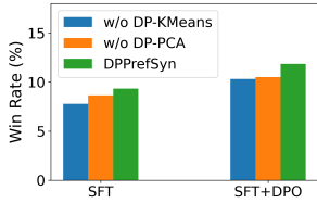
(a) Removing DP-KMeans or DP-PCA.
